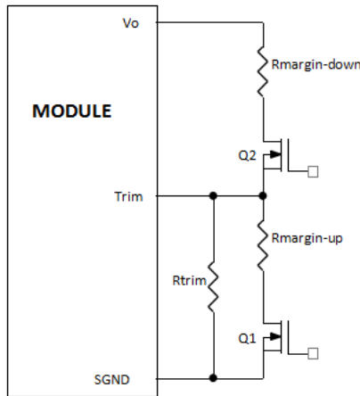
Figure 29. Circuit Configuration for margining Output voltage.
