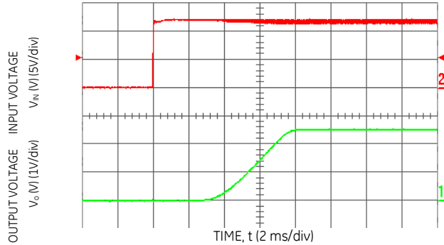
Figure 16. Typical Start-Up with application of V_{in} with low-ESR polymer capacitors at the output ( 7 \times 150\ \mu\text{F} ) ( V_{in} = 12\text{ Vdc} , V_o = 5.0\text{ Vdc} , I_o = 10\text{ A} , C_o = 1050\ \mu\text{F} ).
