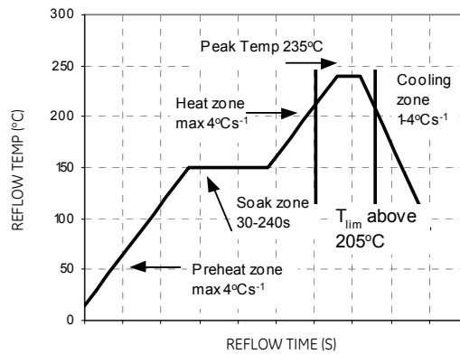
Figure 34. Reflow Profile for Tin/Lead (Sn/Pb) process.
