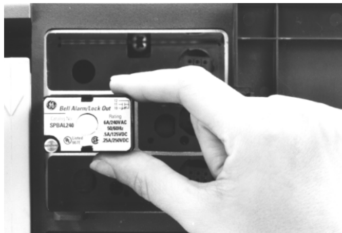
Figure 4. Inserting the Bell Alarm with Lockout into the accessory compartment.
