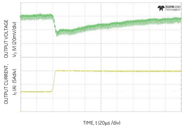
Figure 34. Transient Response to Dynamic Load Change from 50% to 100% at 12Vin, Cout=2x47µF+1x330µF, CTune=2700pF, RTune=300Ω
