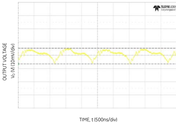
Figure 15. Typical output ripple (Co=2x47µF ceramic, VIN = 12V, Io = Io,max.).
