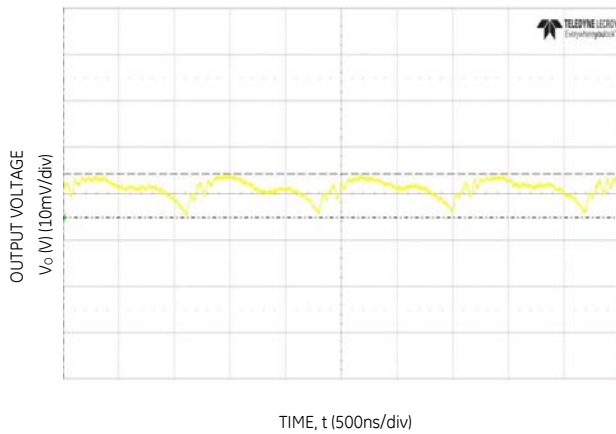
Figure 9. Typical output ripple ( C_0=2 \times 47 \mu\text{F} ceramic, V_{IN} = 12\text{V} , I_o = I_{o,max} ).
