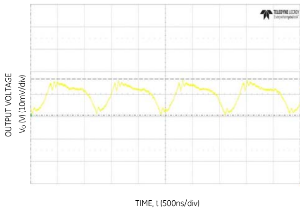
Figure 27. Typical output ripple ( C_o=2 \times 47 \mu\text{F} ceramic, V_{IN} = 12\text{V} , I_o = I_{o,max} ).
