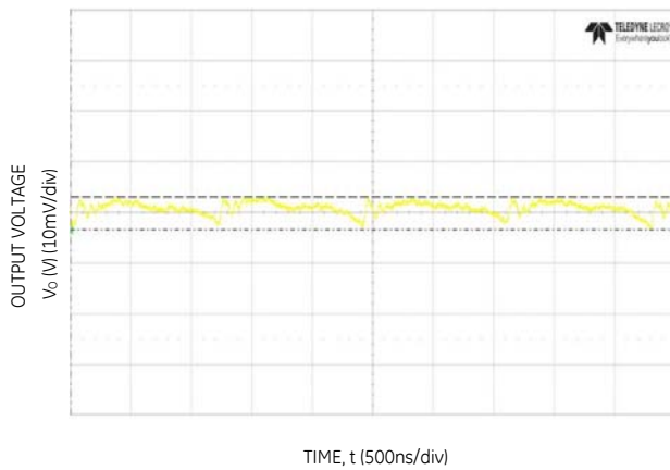
Figure 3. Typical output ripple (Co=2x47µF ceramic, VIN = 12V, Io = Io,max.).
