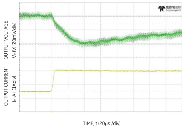
Figure 22. Transient Response to Dynamic Load Change from 50% to 100% at 12Vin, Cout=4x47uF+1x330uF, CTune=10nF, RTune=300Ω
