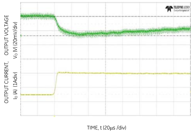
Figure 16. Transient Response to Dynamic Load Change from 50% to 100% at 12Vin, Cout=4x47µF+1x330µF, CTune=15nF, RTune=300
