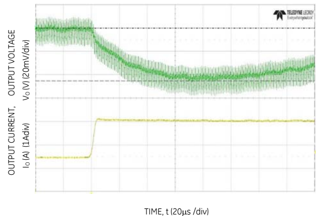
Figure 28. Transient Response to Dynamic Load Change from 50% to 100% at 12Vin, C_{out}=2 \times 47 \mu\text{F} + 1 \times 330 \mu\text{F} , C_{Tune}=6800 \text{pF} , R_{Tune}=300
