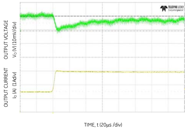
Figure 10. Transient Response to Dynamic Load Change from 50% to 100% at 12Vin, C_{out}=6 \times 47 \mu\text{F} + 1 \times 330 \mu\text{F} , C_{Tune}=5600\text{pF} , R_{Tune}=300 \Omega
