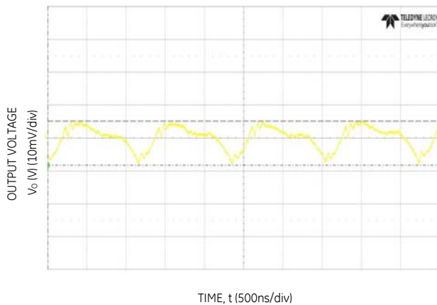
Figure 21. Typical output ripple (Co=2x47µF ceramic, VIN = 12V, Io = Io,max.).
