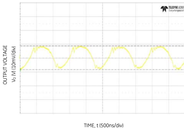
Figure 33. Typical output ripple (Co=2x47µF ceramic, VIN = 12V, Io = Io,max.).
