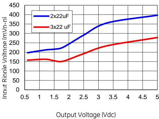
Figure 37. Input ripple voltage for various output voltages with 2x22 µF or 3x22 µF ceramic capacitors at the input (20A load). Input voltage is 12V.
