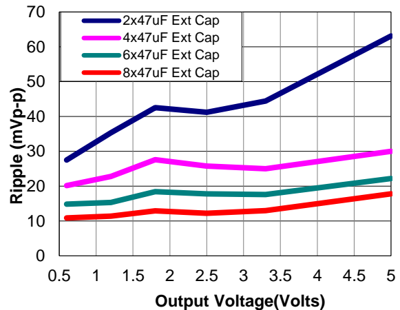
Figure 38. Output ripple voltage for various output voltages with external 2x47 µF, 4x47 µF or 6x47 µF ceramic capacitors at the output (20A load). Input voltage is 12V.
