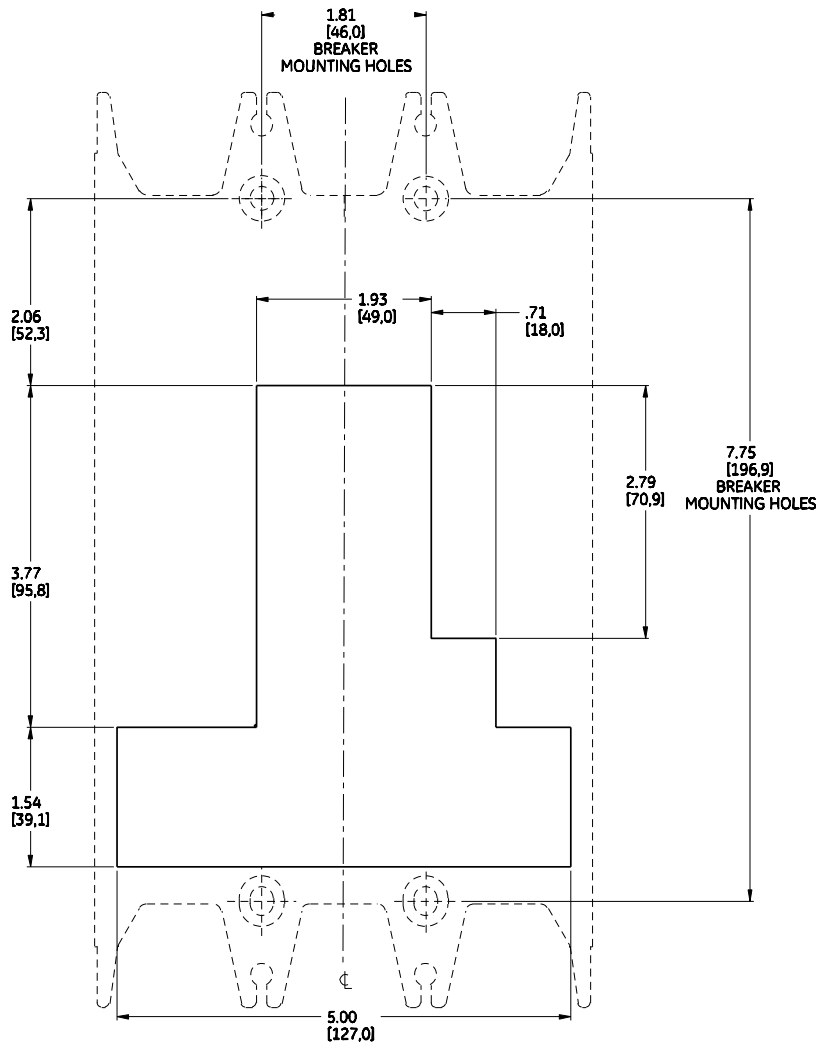
RECOMMENDED DOOR CUTOUT
