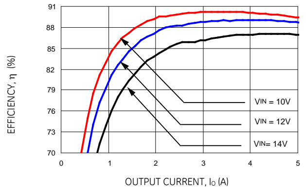
Figure 5. Converter Efficiency versus Output Current (Vout = 3.3Vdc).
