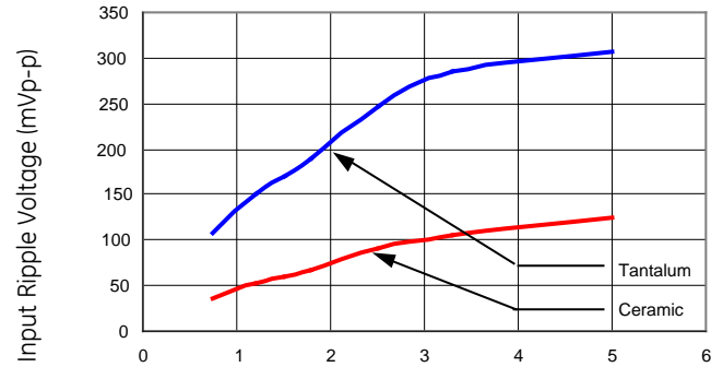
Figure 26. Input ripple voltage for various output with 2x47 µF tantalum capacitors and with 2x22 µF ceramic capacitors at the input (80% of I_{O,max} ).
