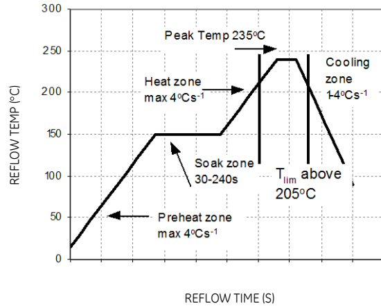
Figure 34. Reflow Profile for Tin/Lead (Sn/Pb) process.
