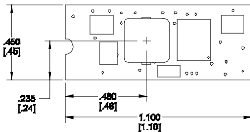
Figure 33. Pick and Place Location.
