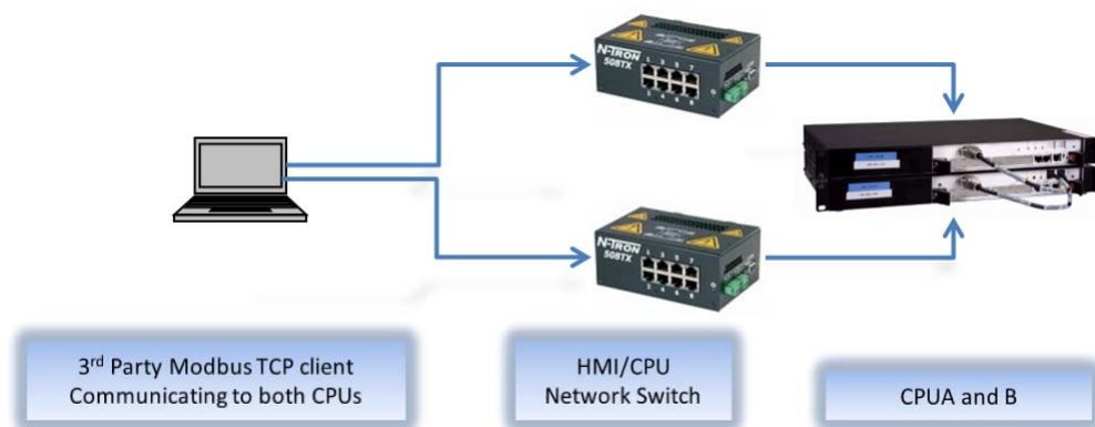
Figure 1-4 Typical 3rd party redundant network configuration
