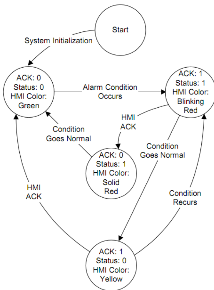
Alarm State Transition Diagram
