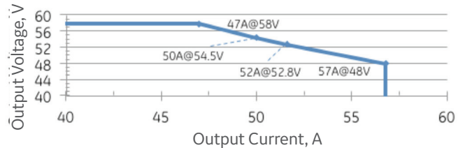
Constant Power to 48 Volts
