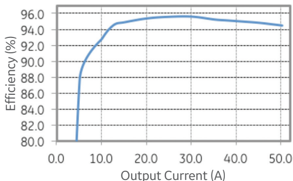
Efficiency vs. Output Current (Temp: 25C, Vin: 240Vac, 60Hz)
