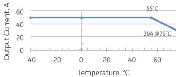
Rated Output Current (at V_{in} > 175V_{ac} )
