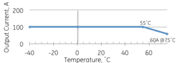
Rated Output Current (at V_{in} > 175V_{ac} )
