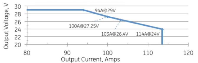
Rated Output Current (at V_{in} > 175V_{ac} )
