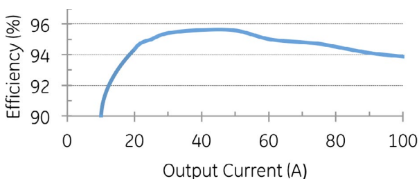
Efficiency % Typical at 240V ac
