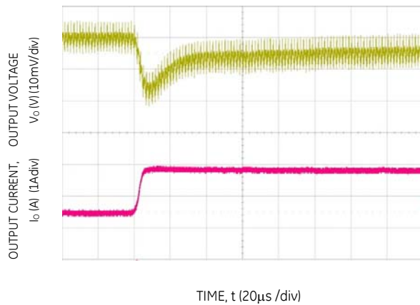
Figure 10. Transient Response to Dynamic Load Change from 50% to 100% at 12Vin, Cout= 1x47µF+1x330µF, CTune=10nF & RTune=267
