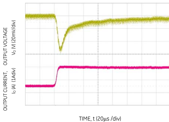
Figure 28 Transient Response to Dynamic Load Change from 50% to 100% at 12V in , C out = 2x47µF, C Tune =2200pF & R Tune =267
