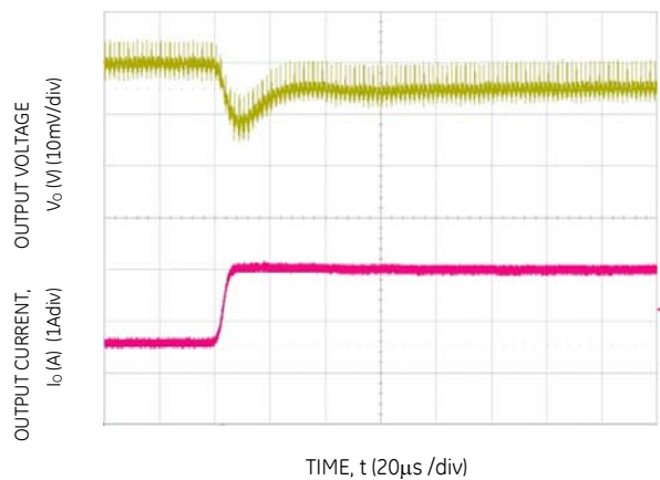
Figure 4. Transient Response to Dynamic Load Change from 50% to 100% at 12Vin, Cout= 1x47uF+2x330uF, CTune=27nF, RTune=180
