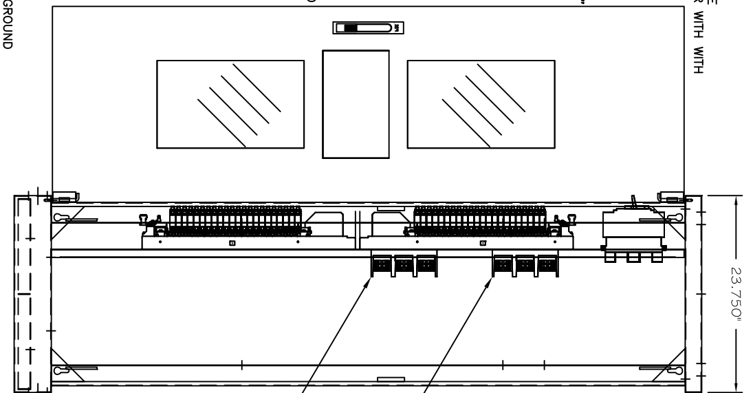
SIDE VIEW (DOOR & COVERS REMOVED)
