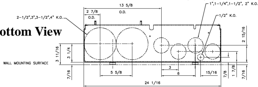
BOTTOM ENDWALL KNOCKOUTS 1.5 X SCALE
